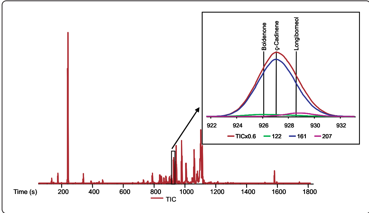
Total Ion Chromatogram (TIC) for the analysis of a ginger oil sample. The inset shows the overlap of three analytes under a single TIC peak.
