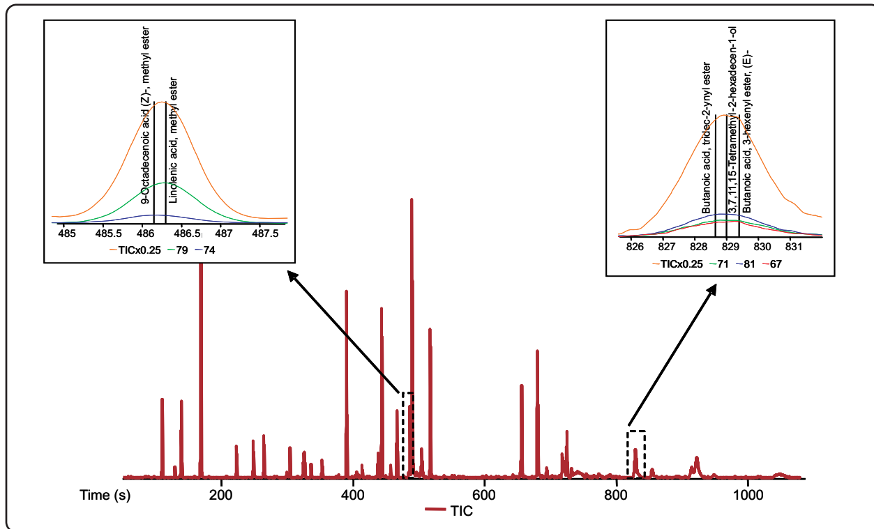
Total Ion Chromatogram (TIC) for the analysis of a jasmine oil sample. The insets show examples of deconvolution for analytes that are not chromatographically resolved.
